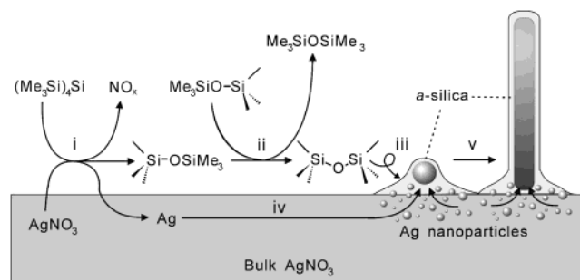
Scheme 1. Proposed Reaction Steps To Form \alpha -Silica Shell Encapsulated Ag Nanowires
